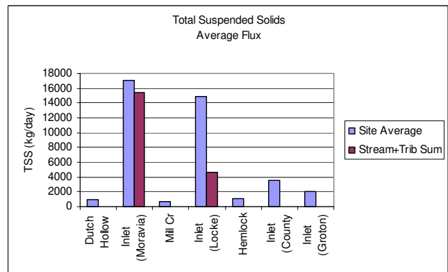
Fig. 25. Site averaged total suspended solids flux.
