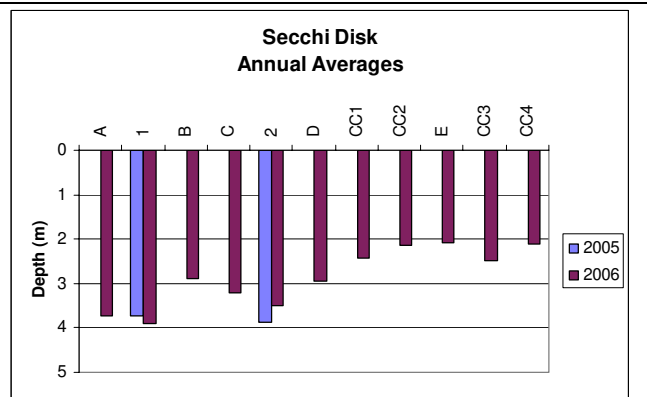
Fig. 13. Site averaged secchi disk depths.
