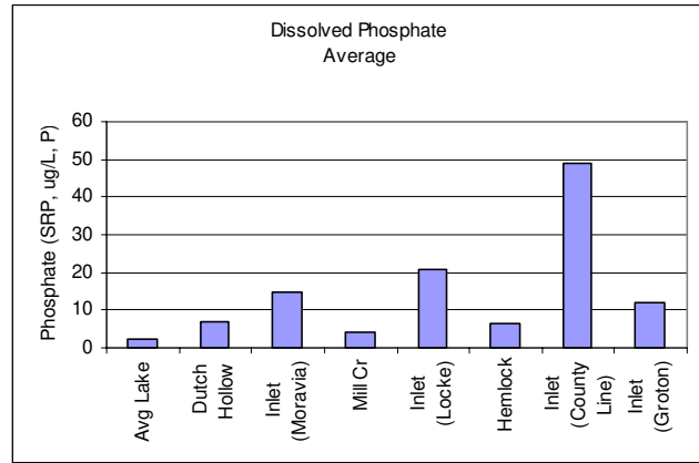
Fig. 19. Site averaged dissolved phosphate.
