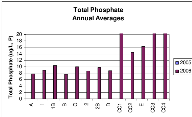
Fig. 8. Site averaged total phosphate. “B” designates the bottom water sample. CC1 = 94, CC3 = 125, CC4 = 607
