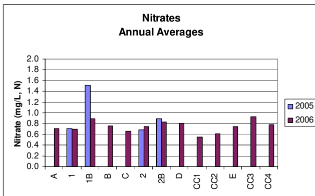
Fig. 10. Site averaged nitrate. “B” designates the bottom water sample.
