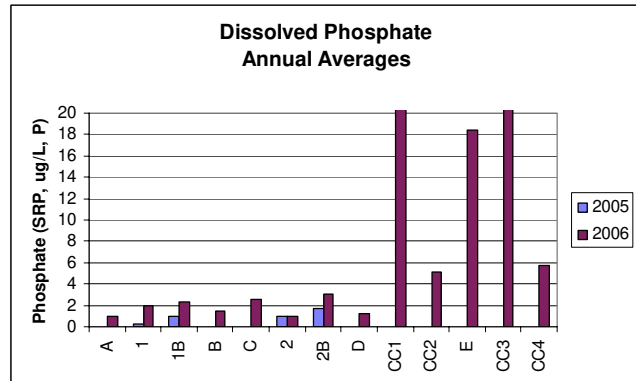
Fig. 9. Site averaged dissolved phosphate. “B” designates the bottom water sample. CC1 = 97, CC3 = 80.
