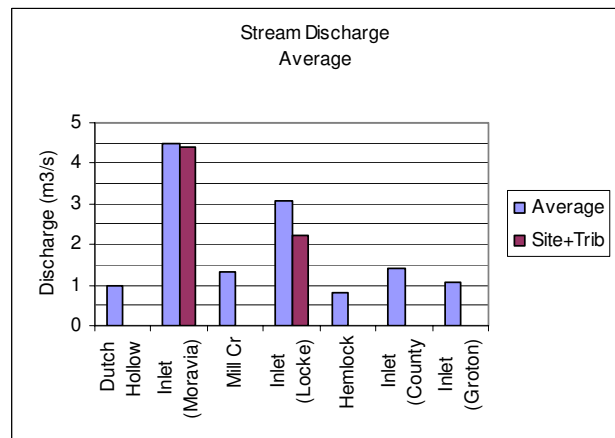
Fig. 17. Site averaged stream discharge.
