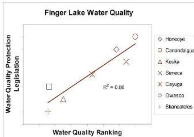
Fig. 1. The 2005 water ranking of seven Finger Lakes.
