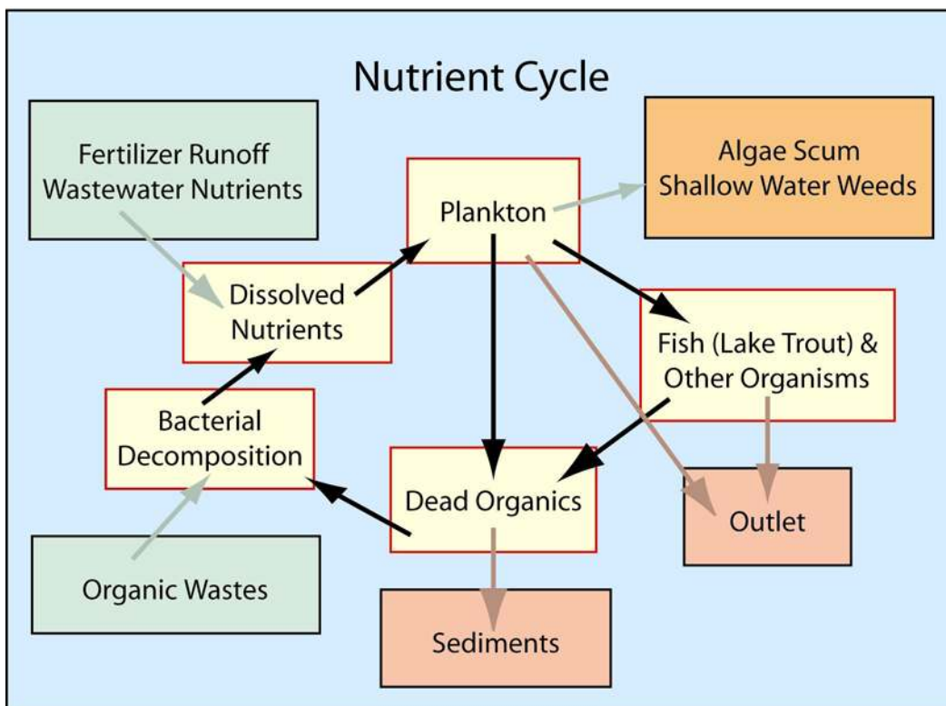
Fig. 3. A typical nutrient cycle for lake ecosystems (yellow boxes). Typical human-induced additions (green boxes) to, their impact (orange box), and natural sinks (red boxes) from the nutrient cycle are also shown.
