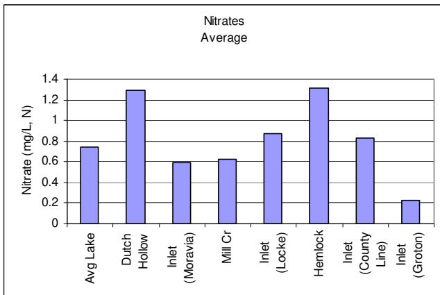
Fig. 20. Site averaged nitrate.
