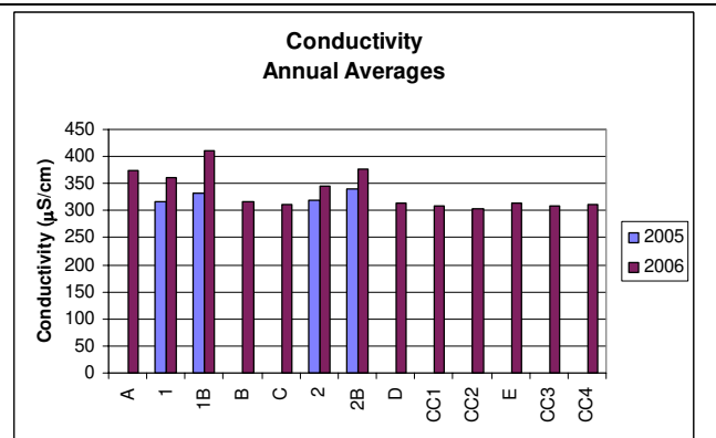
Fig. 15. Site averaged conductivity (specific conductance). "B" designates the bottom water sample.
