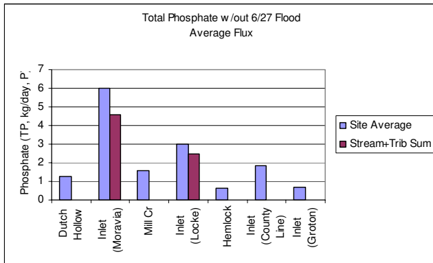
Fig. 22. Site averaged total phosphate flux.
