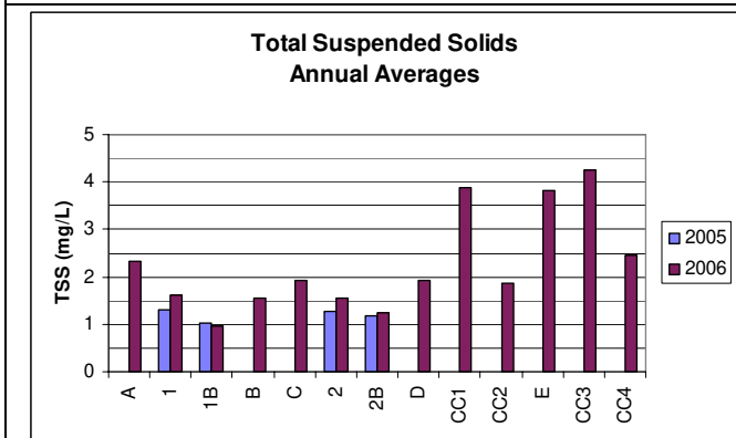
Fig. 14. Site averaged total suspended solids. "B" designates the bottom water sample.
