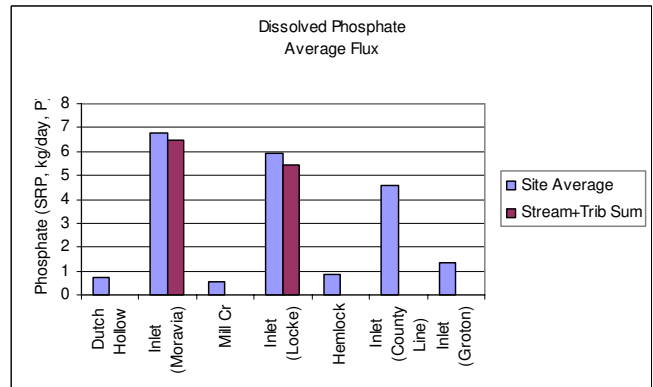
Fig. 23. Site averaged dissolved phosphate flux.
