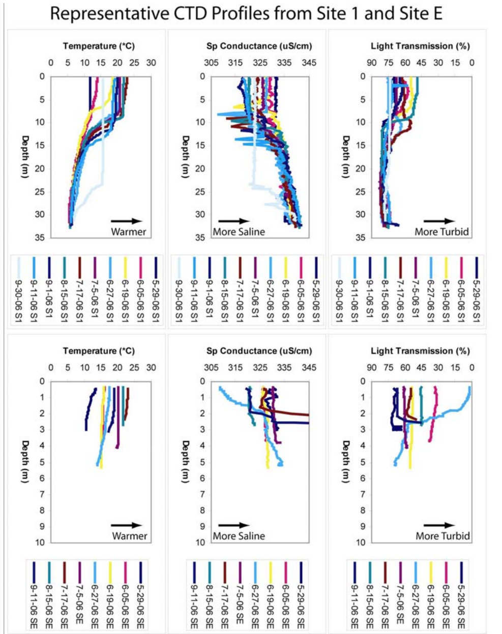
Fig. 6. Representative CTD profiles from Site 1 (open water) and Site E (southern end near Owasco Inlet).
