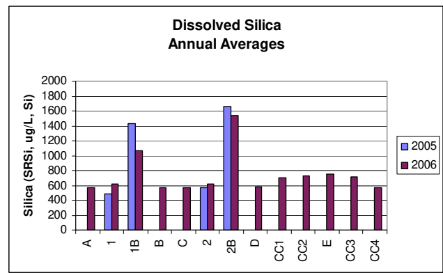
Fig. 11. Site averaged dissolved silica. “B” designates the bottom water sample.
