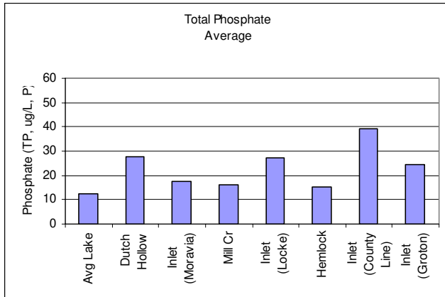
Fig. 18. Site averaged total phosphate.
