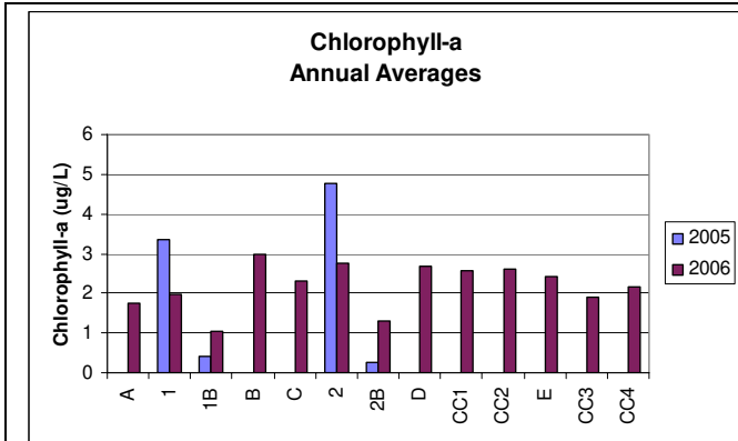
Fig. 12. Site averaged chlorophyll-a. "B" designates the bottom water sample.
