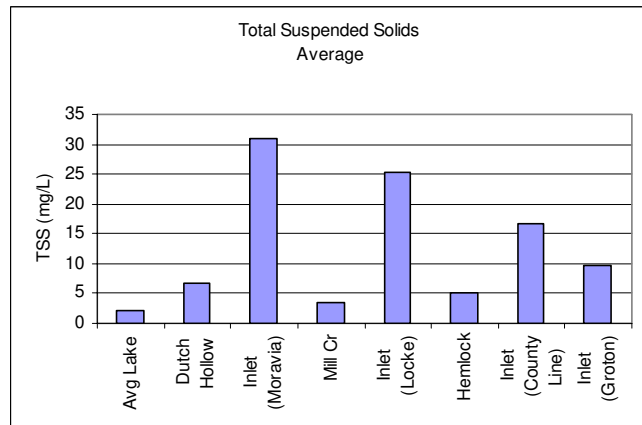
Fig. 21. Site averaged total suspended solids.
